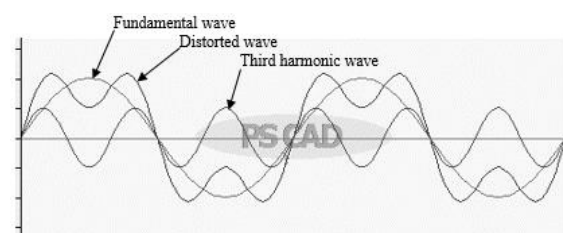
Figure 1. Wave Distorted by Harmonics
