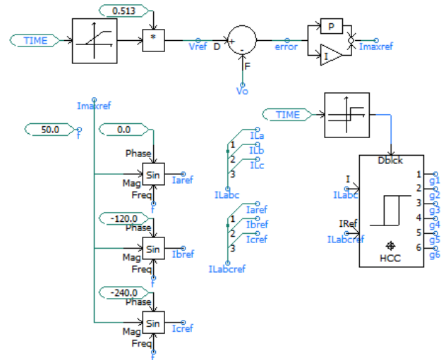
Figure 14. Hysteresis Current Control Circuit in 3-Phase PWM Rectifier
