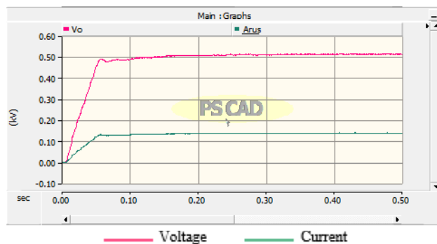
Figure 13. 3-Phase PWM Rectifier Output Waveform
