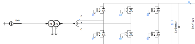
Figure 12. 3-Phase PWM Rectifier Circuit
