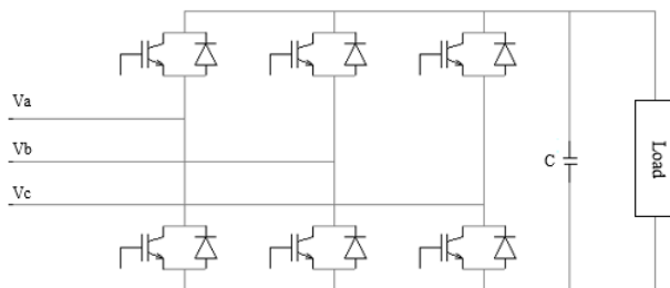
Figure 2. 3-Phase PWM Rectifier Topology
