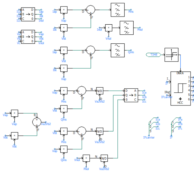
Figure 19. Active Filter Control Circuit Based on P-Q Theory
