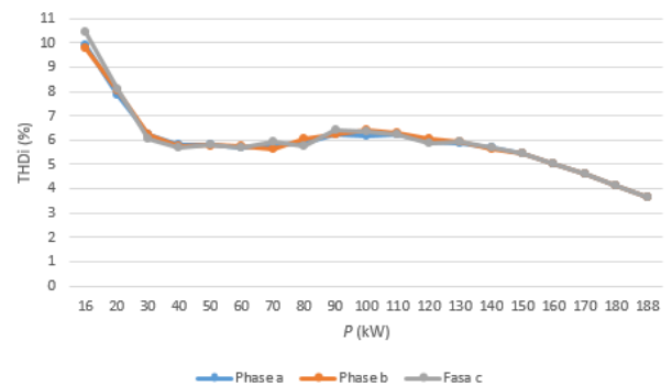
Figure 17. Graph of THD i Relationship to the Output Power ( P )
