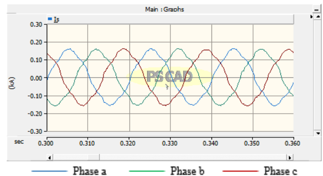
Figure 15. 3-Phase PWM Rectifier Input Current Waveform
