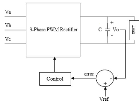
Figure 3. Principle Operation of PWM Rectifier
