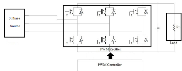
Figure 6. Block Diagram of Distorted System
