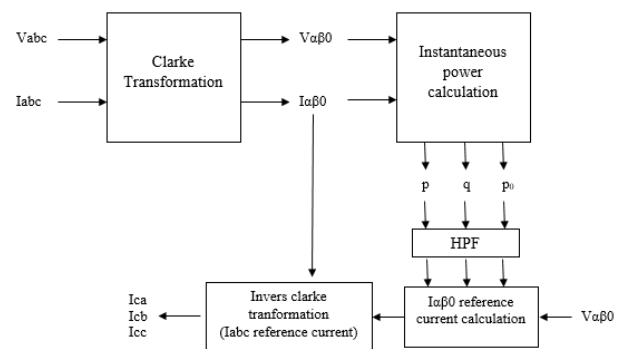
Figure 10. Block Diagram for Active Harmonic Filter Control Based on P-Q theory
