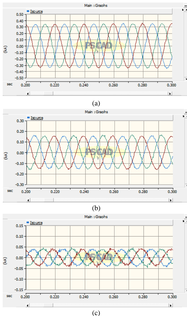
Figure 22. The Input Current of the 3-Phase PWM Rectifier with Active Filter at Power Level, (a) 150 kW, (b) 70 kW, and (c) 16 kW
