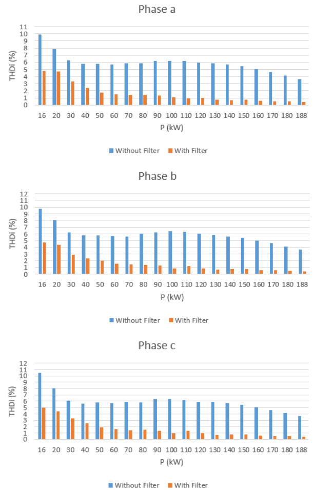
Figure 21. Graph of THD_i Relationship to the Output Power ( P ) Before and After the Application of the Active Filter
