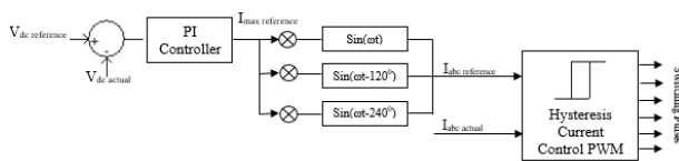
Figure 8. Control Technique of 3-Phase PWM Rectifier
