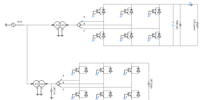
Figure 18. 3-Phase PWM Rectifier Circuit with Active Filter
