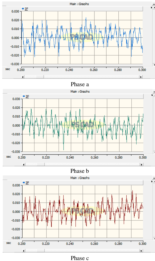
Figure 20. The Compensation Current Waveform for the Three Phases
